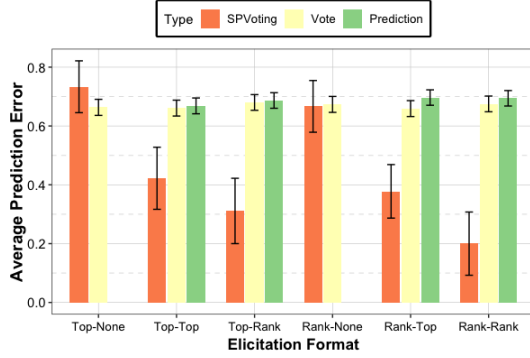
Figure 5: Average error in predicting the top alternative in the ground truth. By combining both the vote and prediction, SP voting achieves a much lower error than in either piece of information.
